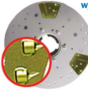
Single Bar PCD Trapezoid KA1800-R
